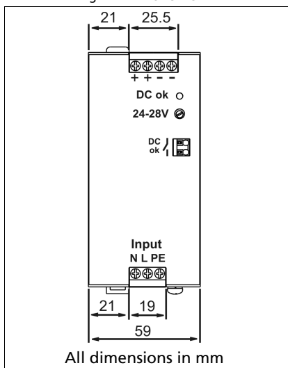
Fig. 21-1 Front view
