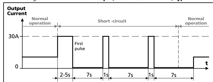
Fig. 6-2 Short-circuit on output, intermittent current, typ.
