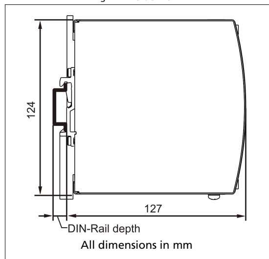
Fig. 21-2 Side view
